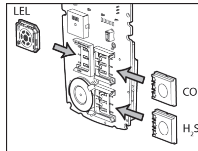
Figure 12. Sensor Positioning
